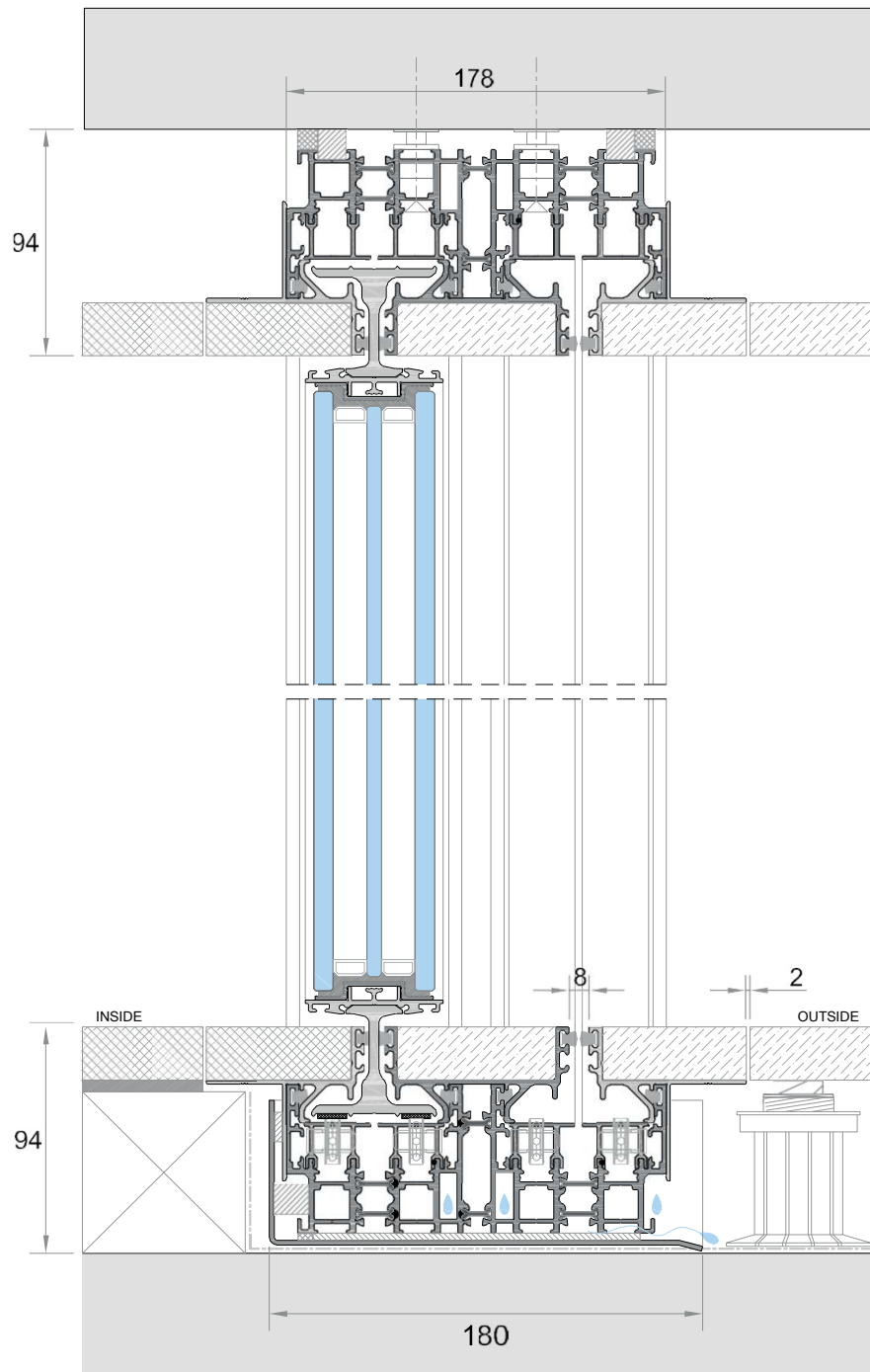
VERTICAL SECTION
