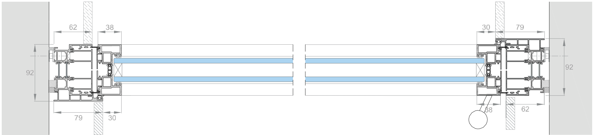
HORIZONTAL SECTION
