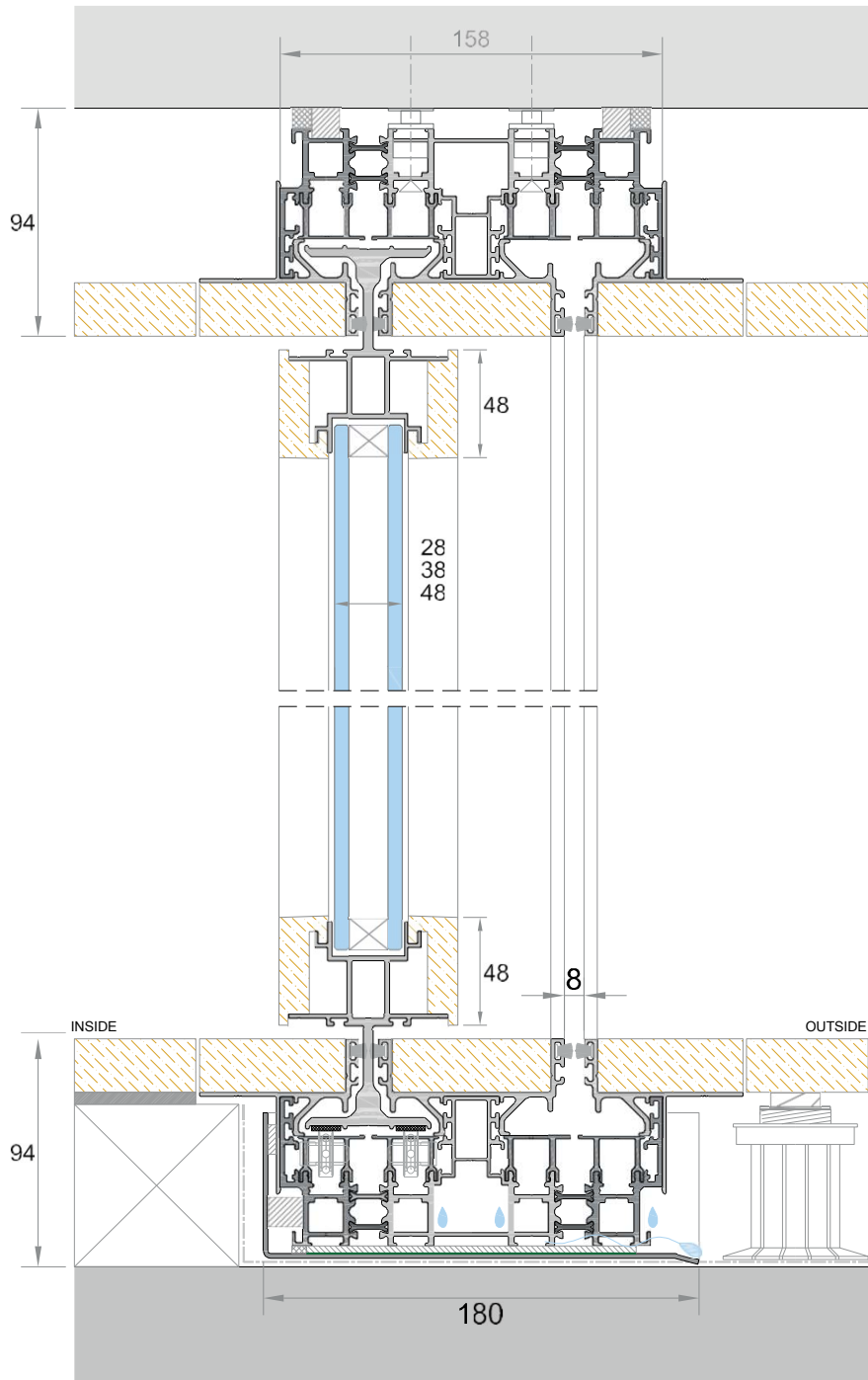
VERTICAL SECTION
