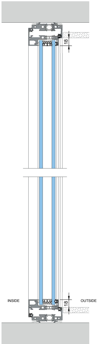
VERTICAL SECTION BB
