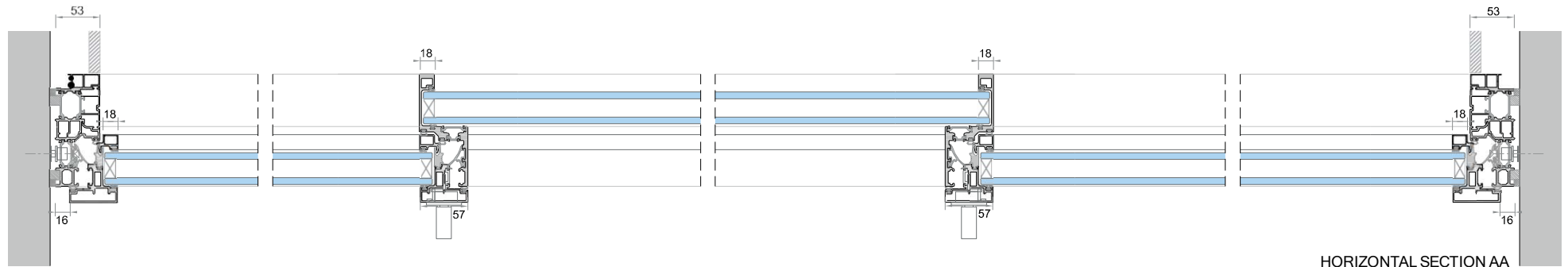
HORIZONTAL SECTION AA
