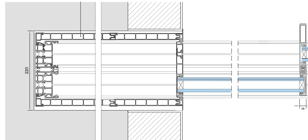
Perimetral aluminium box for hidden sliding windows
