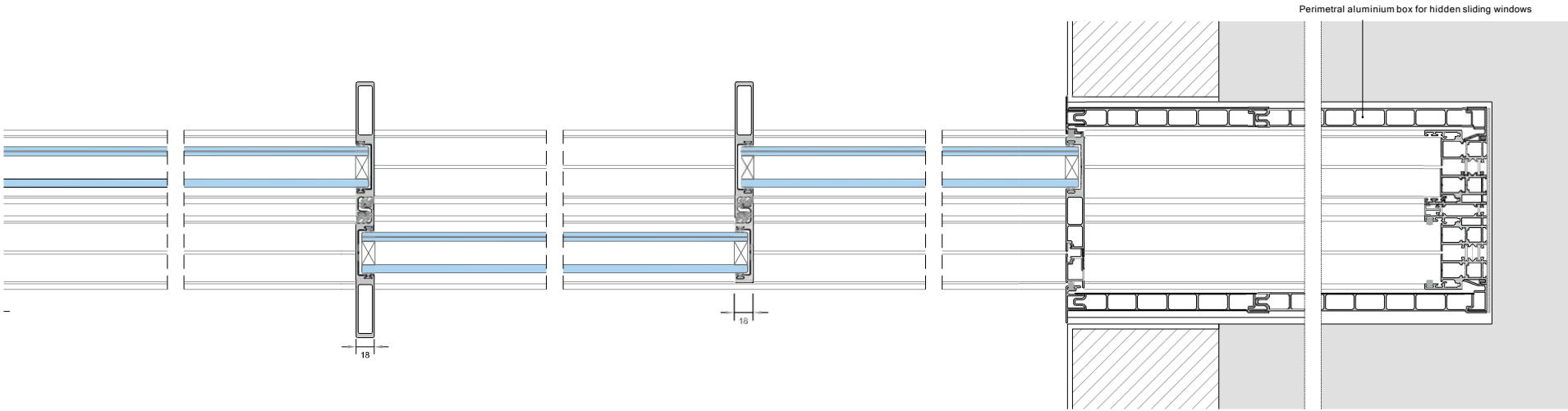
Perimetral aluminium box for hidden sliding windows
