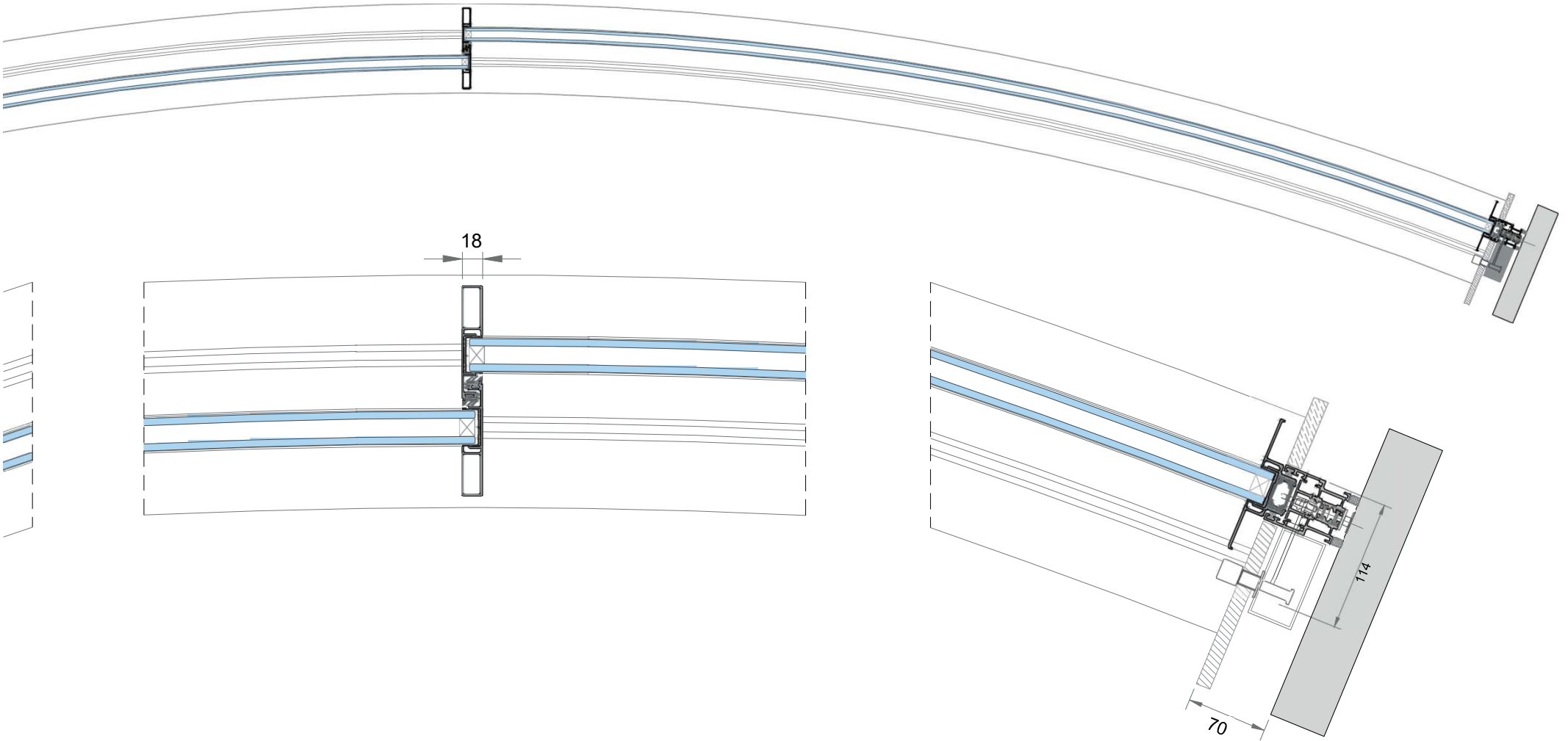
HORIZONTAL SECTION
