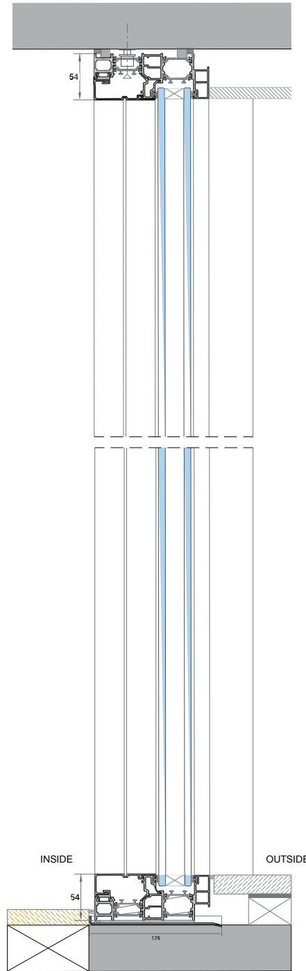
VERTICAL SECTION CC
