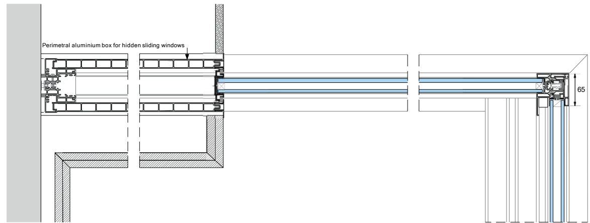
HORIZONTAL SECTION
