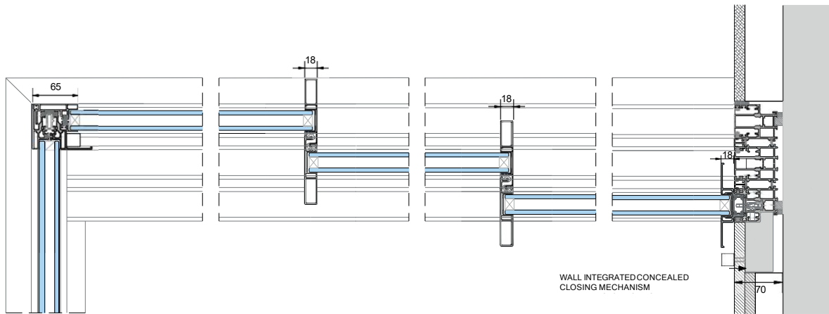
HORIZONTAL SECTION
