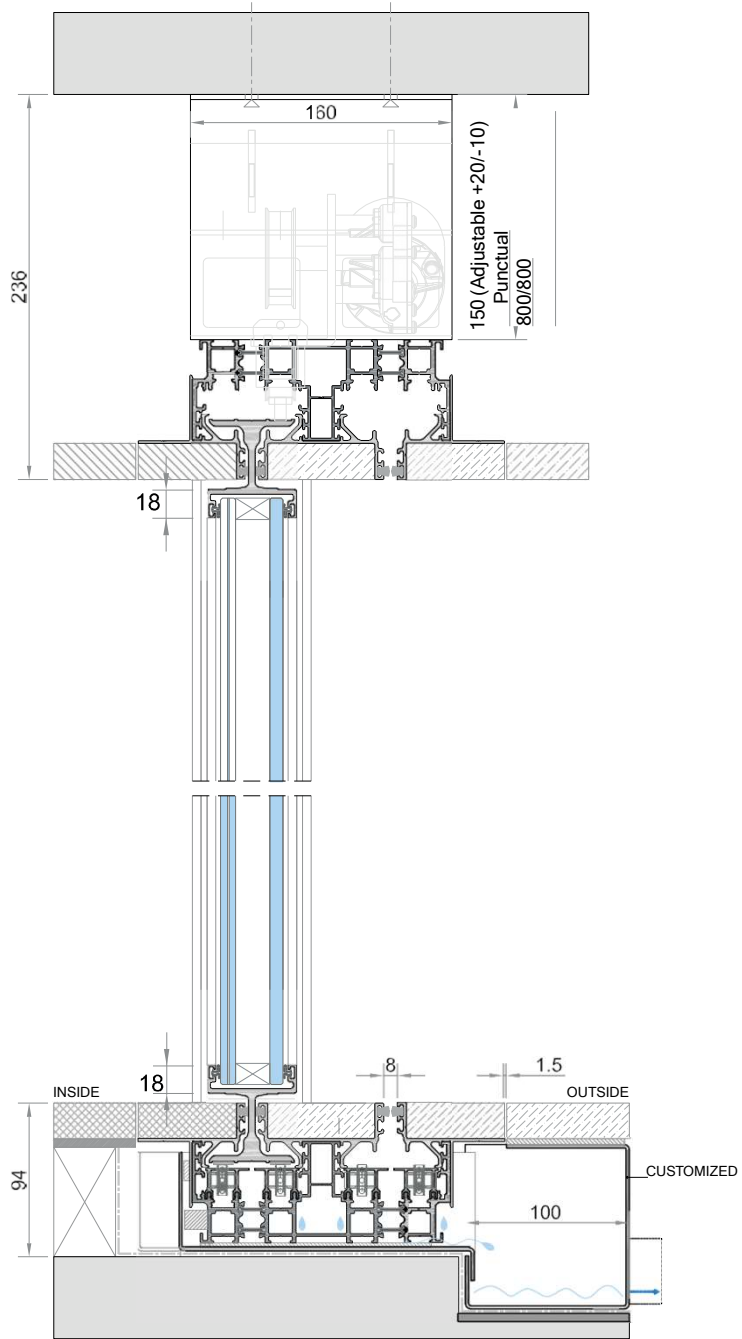
VERTICAL SECTION
