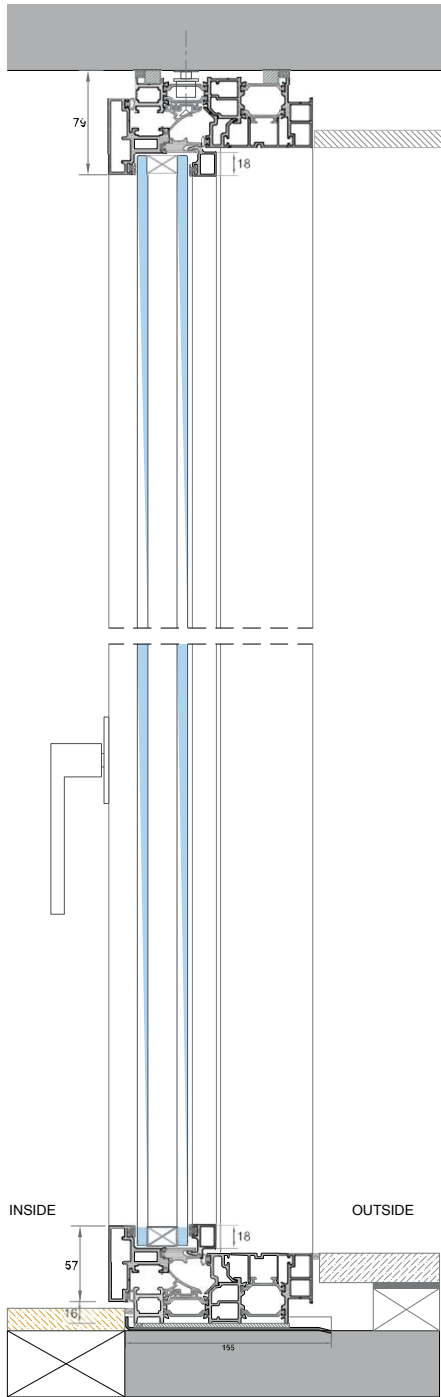
VERTICAL SECTION BB
